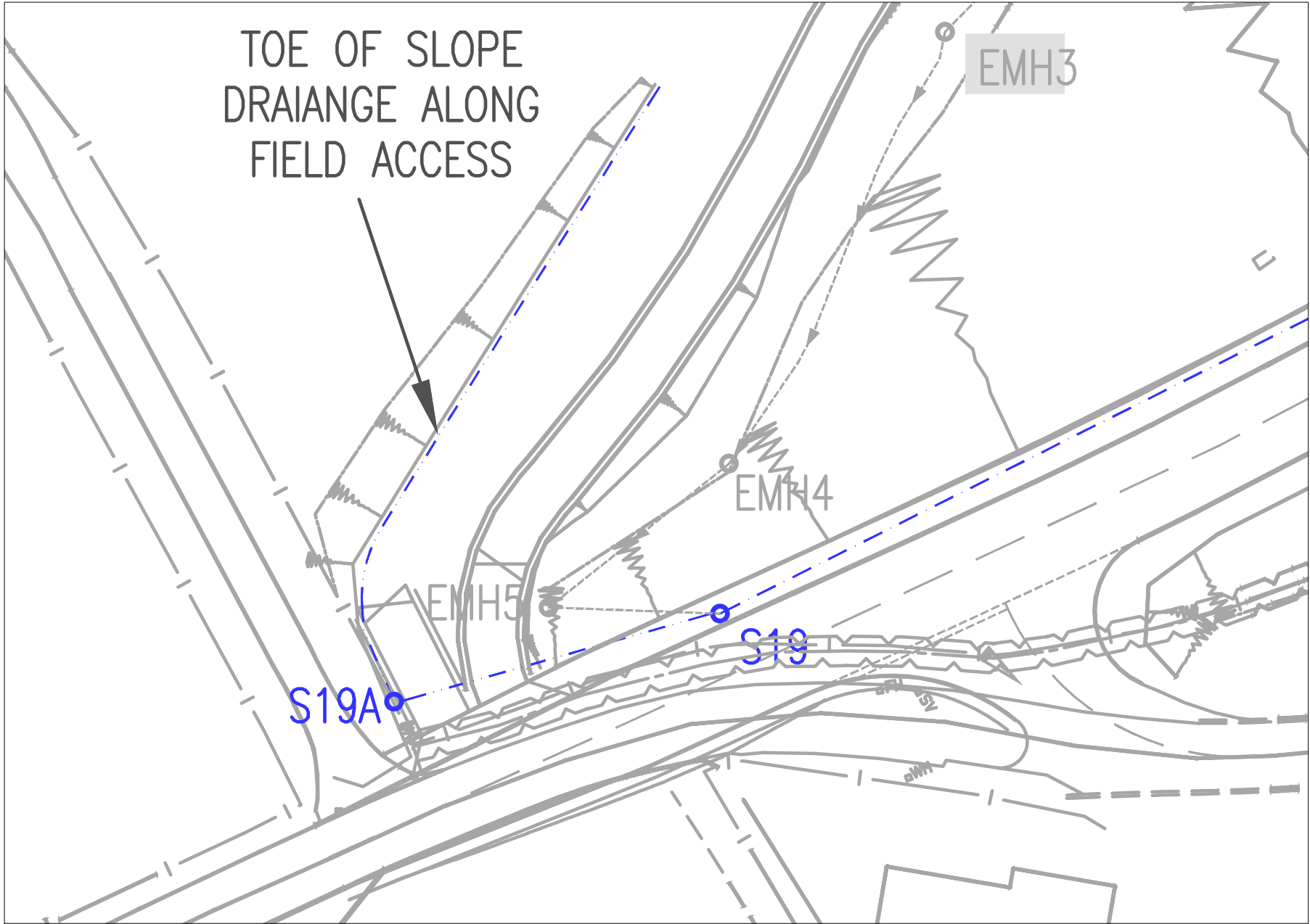
EXTRACT OF DRAINAGE DRAWING - NOT TO SCALE
